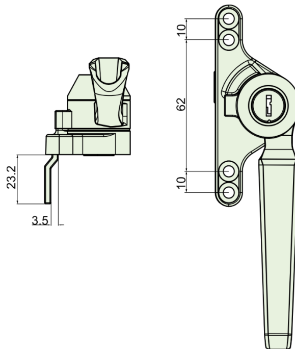
Dimensions with Standard Drive Blade
